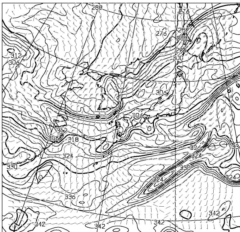
T=36 850hPa: E.P. TEMP(K), WIND(KNOTS) VALID 191200UTC
