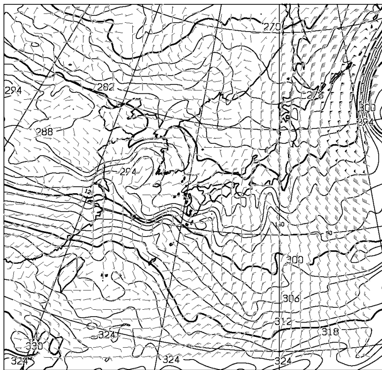
T=24 850hPa: E.P.TEMP(K),WIND(KNOTS) VALID 280000UTC
