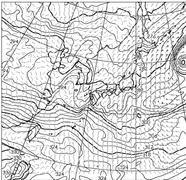
T=12 850hPa: E.P.TEMP(K),WIND(KNOTS) VALID 271200UTC
