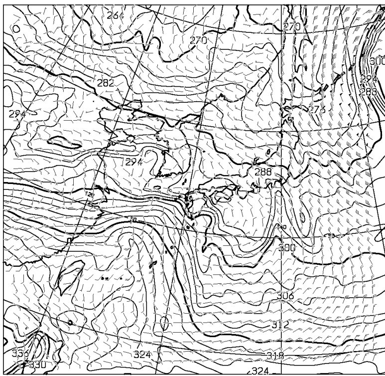
T=36 850hPa: E.P.TEMP(K),WIND(KNOTS) VALID 281200UTC
