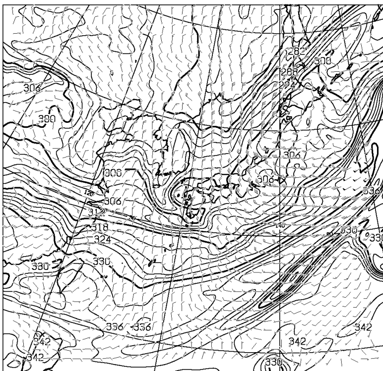
T=48 850hPa: E.P. TEMP(K), WIND(KNOTS) VALID 200000UTC
