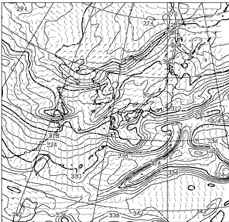
T=24 850hPa: E.P. TEMP(K), WIND(KNOTS) VALID 190000UTC
