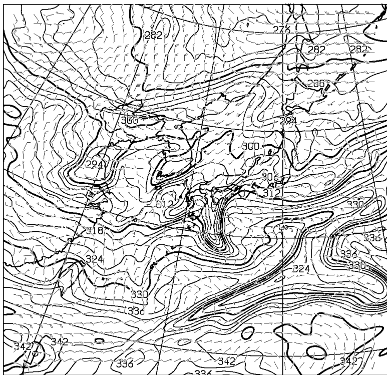
T=12 850hPa: E.P. TEMP(K), WIND(KNOTS) VALID 181200UTC
