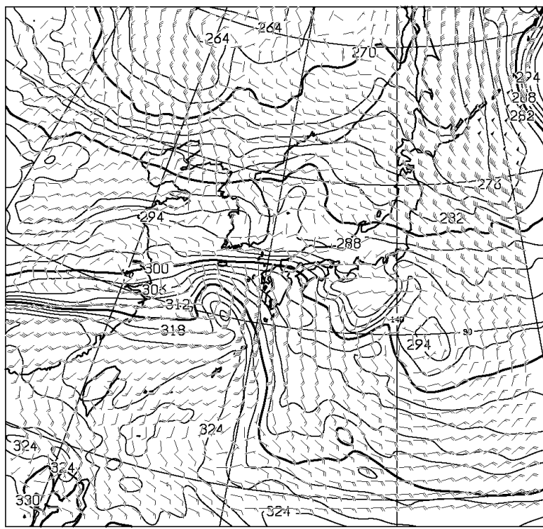
T=48 850hPa: E.P.TEMP(K),WIND(KNOTS) VALID 290000UTC
