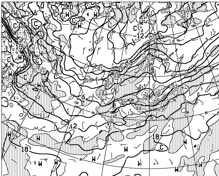
T=36 VALID 190000UTC TEMP (C), WIND ARROW AT 850hPa P-VEL (hPa/h) AT 700hPa
