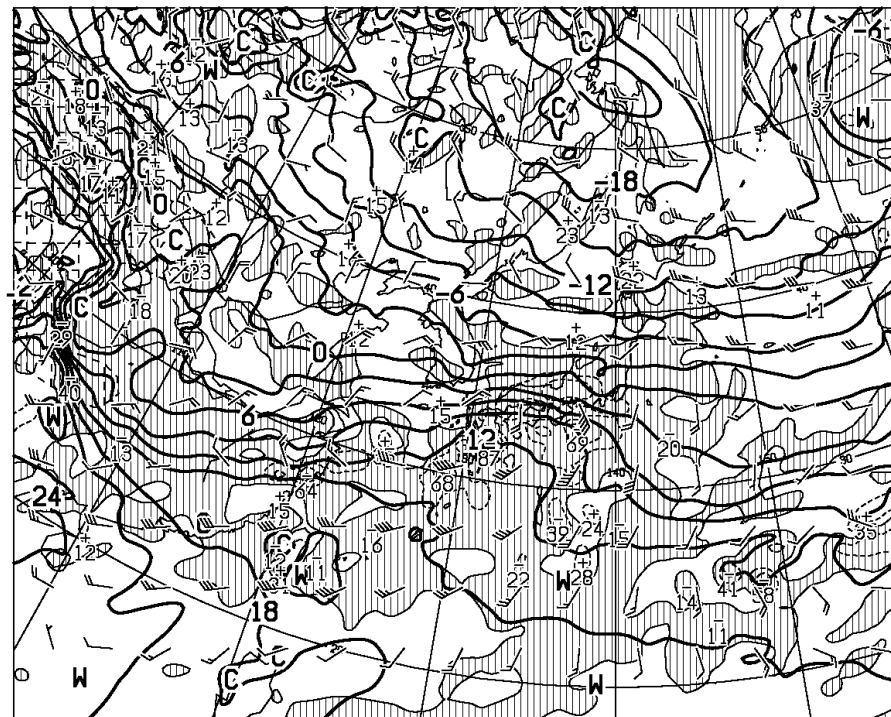
T=48 VALID 051200UTC TEMP(C), WIND ARROW AT 850hPa P-VEL(hPa/h) AT 700hPa
