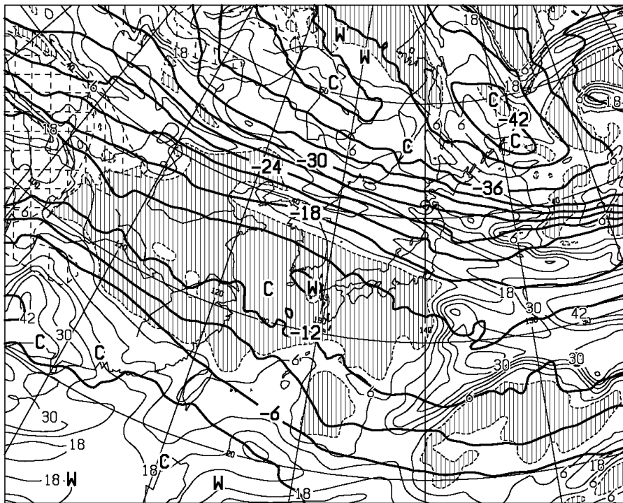
T=36 VALID 050000UTC TEMP(C) AT 500hPa T-TD(C) AT 700hPa
