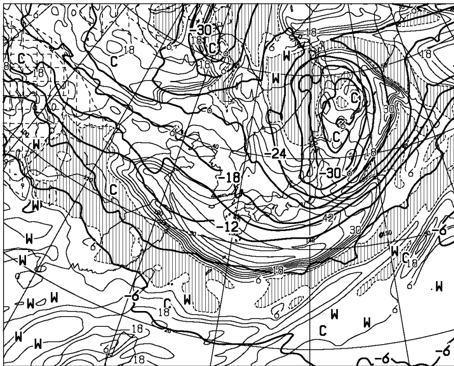
T=36 VALID 261200UTC TEMP( C) AT 500hPa T-TD( C) AT 700hPa
