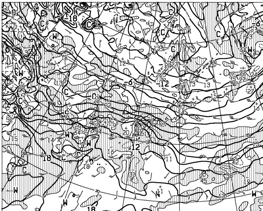
T=36 VALID 050000UTC TEMP(C), WIND ARROW AT 850hPa P-VEL(hPa/h) AT 700hPa
