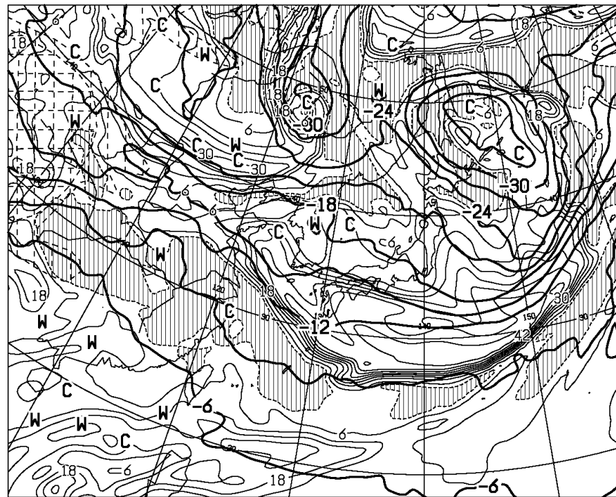
T=48 VALID 270000UTC TEMP( C) AT 500hPa T-TD( C) AT 700hPa
