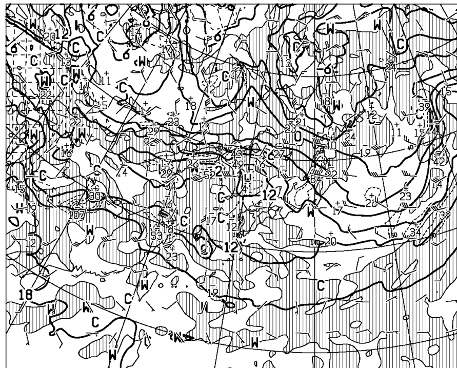
T=48 VALID 270000UTC TEMP( C), WIND ARROW AT 850hPa P-VEL(hPa/h) AT 700hPa
