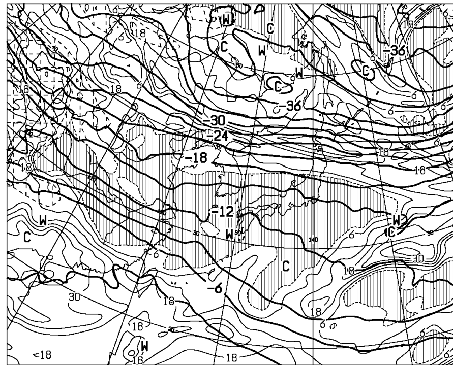
T=48 VALID 051200UTC TEMP(C) AT 500hPa T-TD(C) AT 700hPa
