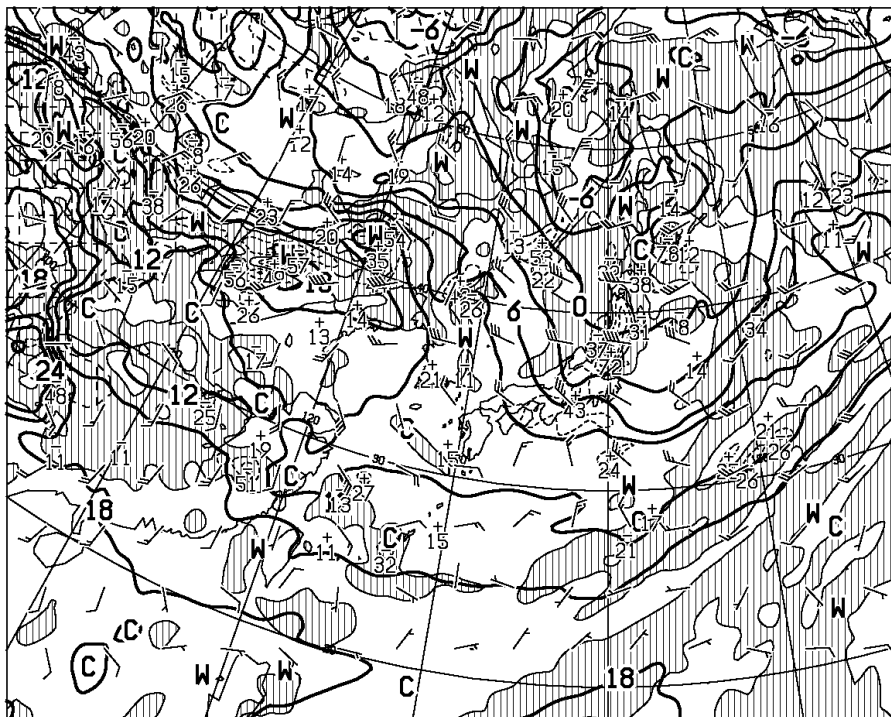
T=36 VALID 261200UTC TEMP( C), WIND ARROW AT 850hPa P-VEL(hPa/h) AT 700hPa
