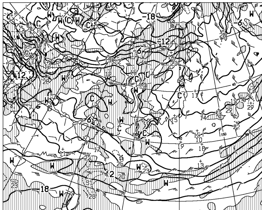
T=24 VALID 281200UTC TEMP (C), WIND ARROW AT 850hPa P-VEL (hPa/h) AT 700hPa
