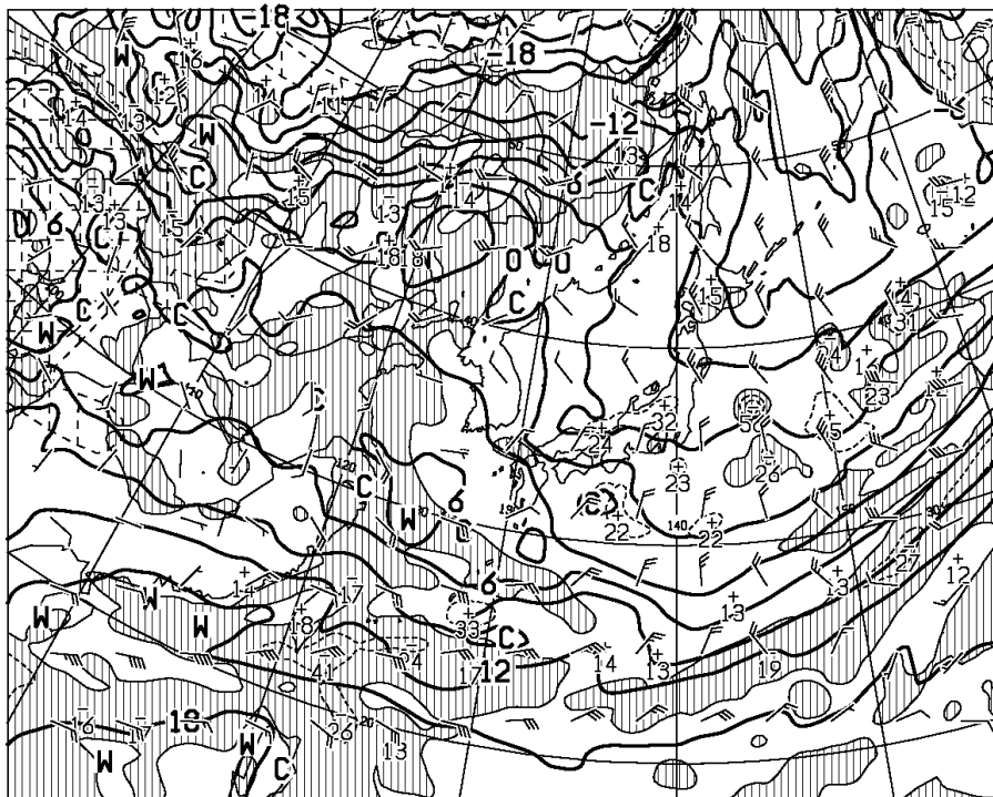
T=12 VALID 280000UTC TEMP (C), WIND ARROW AT 850hPa P-VEL (hPa/h) AT 700hPa
