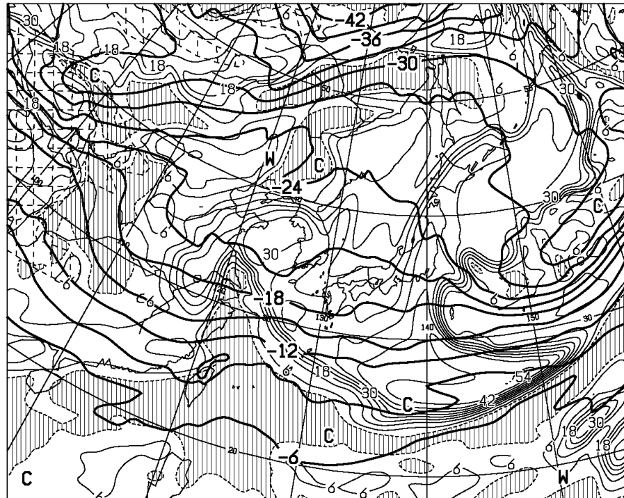
T=24 VALID 281200UTC TEMP (C) AT 500hPa T-TD (C) AT 700hPa
