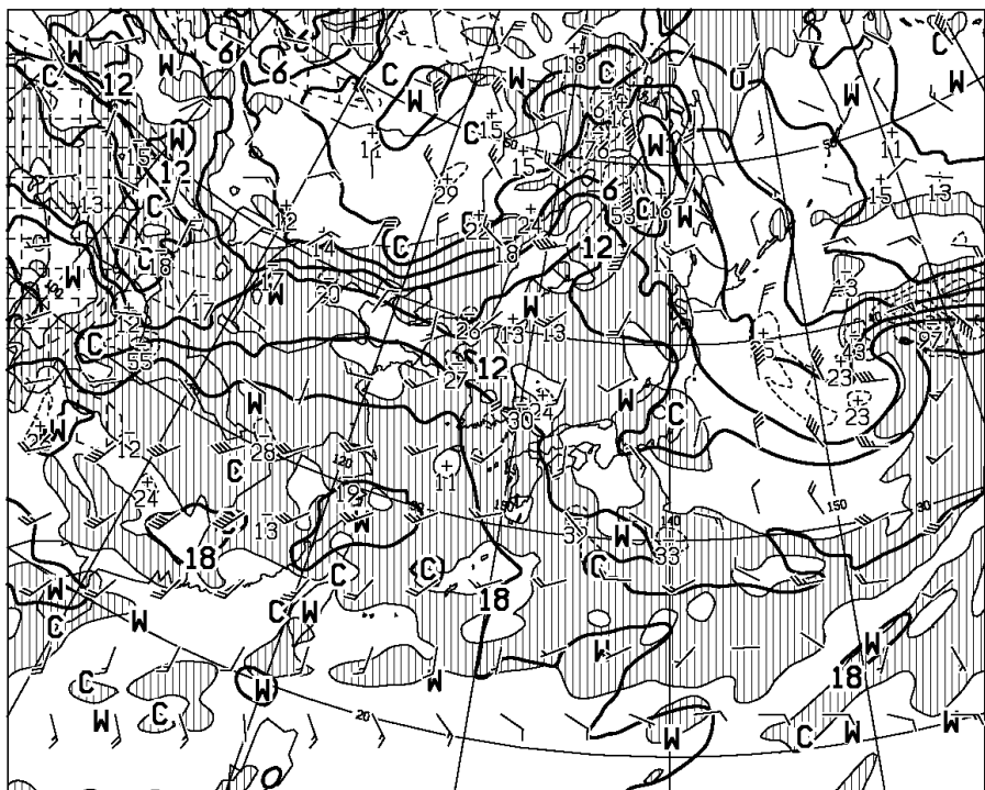
T=12 VALID 150000UTC TEMP (C), WIND ARROW AT 850hPa P-VEL (hPa/H) AT 700hPa
