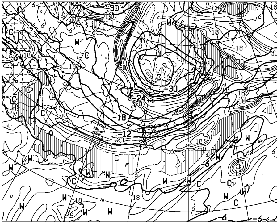
T=12 VALID 251200UTC TEMP (C) AT 500hPa T-TD (C) AT 700hPa
