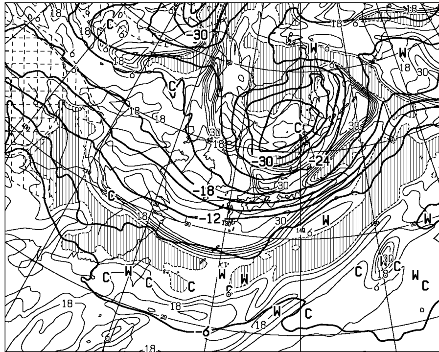
T=24 VALID 260000UTC TEMP (C) AT 500hPa T-TD (C) AT 700hPa
