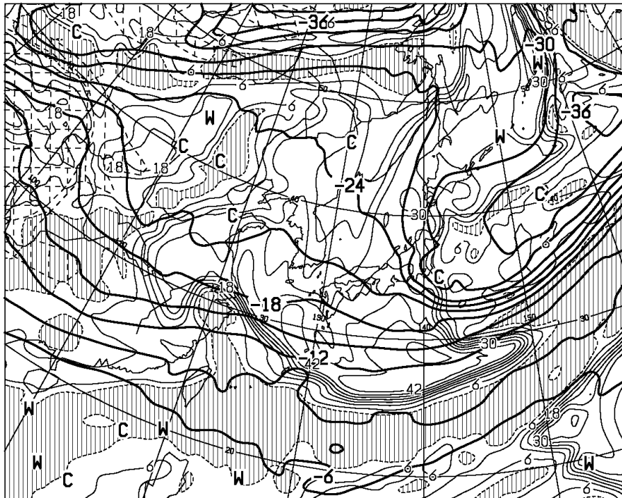
T=12 VALID 280000UTC TEMP (C) AT 500hPa T-TD (C) AT 700hPa
