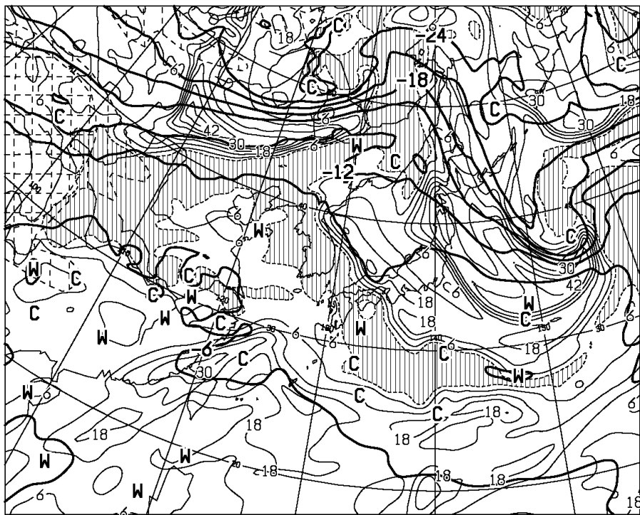
T=12 VALID 150000UTC TEMP (C) AT 500hPa T-TD (C) AT 700hPa
