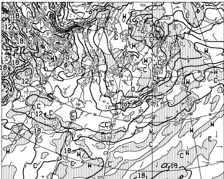
T=12 VALID 251200UTC TEMP (C), WIND ARROW AT 850hPa P-VEL (hPa/H) AT 700hPa
