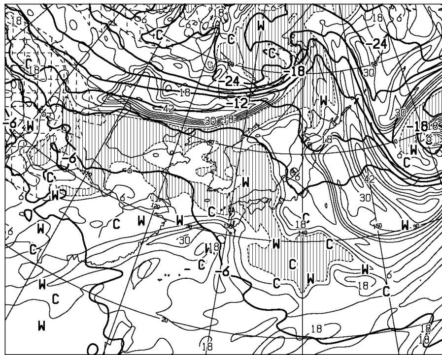
T=24 VALID 151200UTC TEMP (C) AT 500hPa T-TD (C) AT 700hPa
