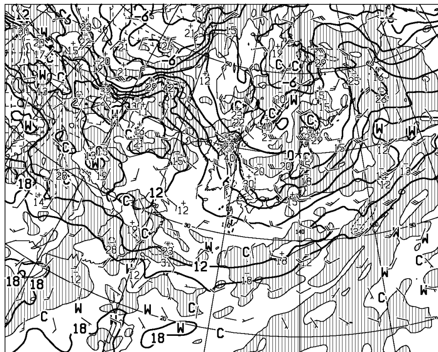
T=24 VALID 260000UTC TEMP (C), WIND ARROW AT 850hPa P-VEL (hPa/H) AT 700hPa
