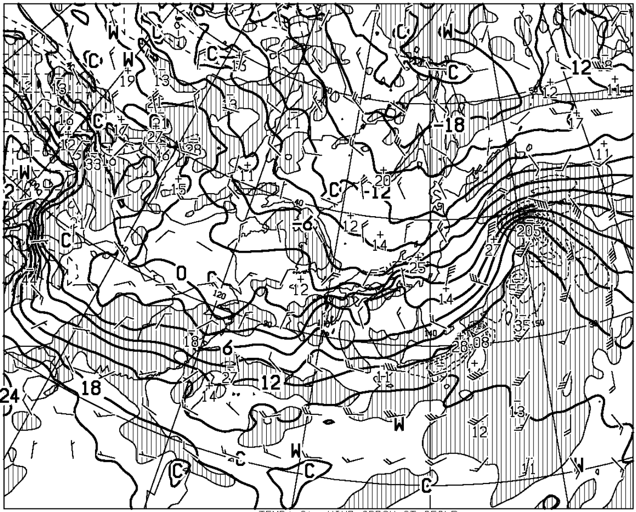
T=72 VALID 061200UTC TEMP (C), WIND ARROW AT 850hPa P-VEL (hPa/H) AT 700hPa
