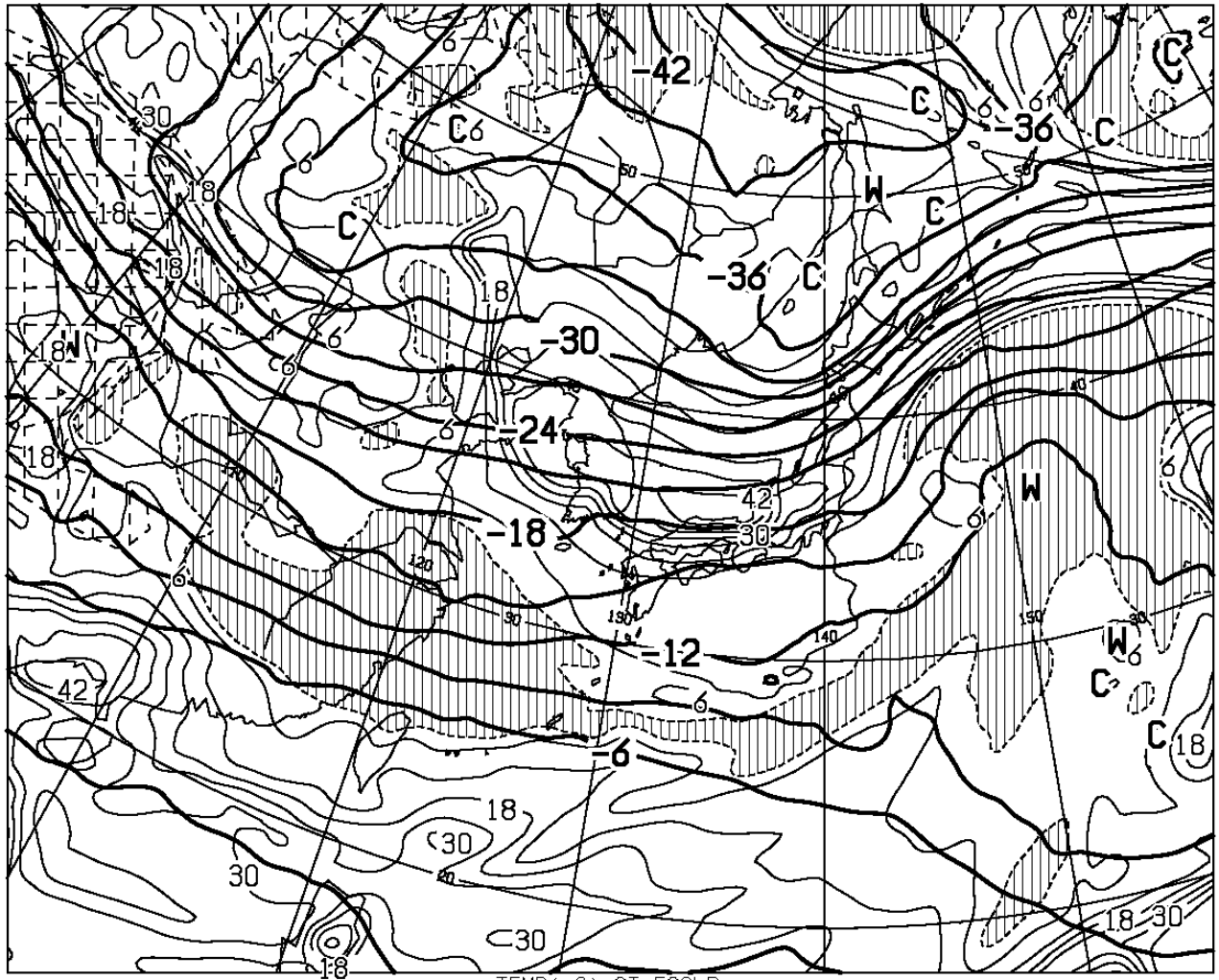
T=72 VALID 061200UTC TEMP (C) AT 500hPa T-TD (C) AT 700hPa
