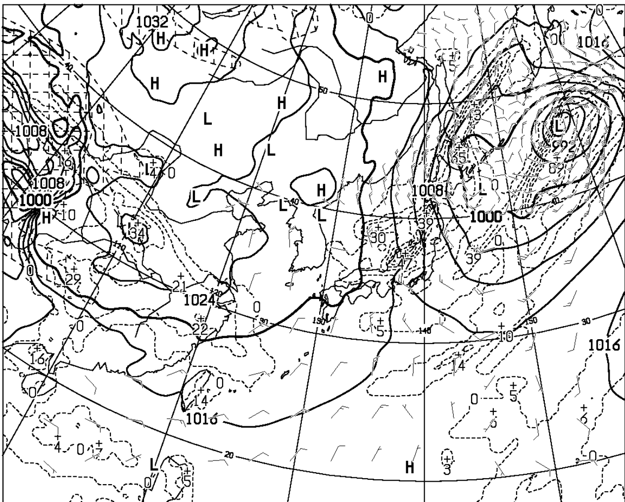
T=72 VALID 201200UTC SURFACE PRESS (hPa), PRECIP (MM) (48-72) WIND ARROW AT SURFACE
