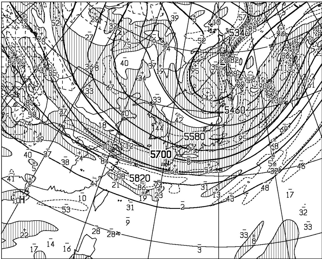
T=72 VALID 201200UTC HEIGHT (M), VORT (10** \times -6/SEC) AT 500hPa
