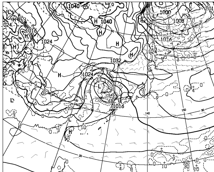
T=48 VALID 111200UTC SURFACE PRESS (hPa), PRECIP (MM) (36-48) WIND ARROW AT SURFACE
