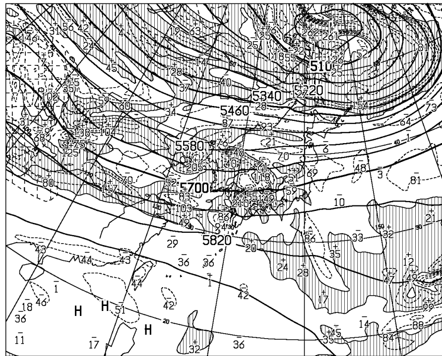
T=48 VALID 111200UTC HEIGHT (M), VORT (10** -6 /SEC) AT 500hPa
