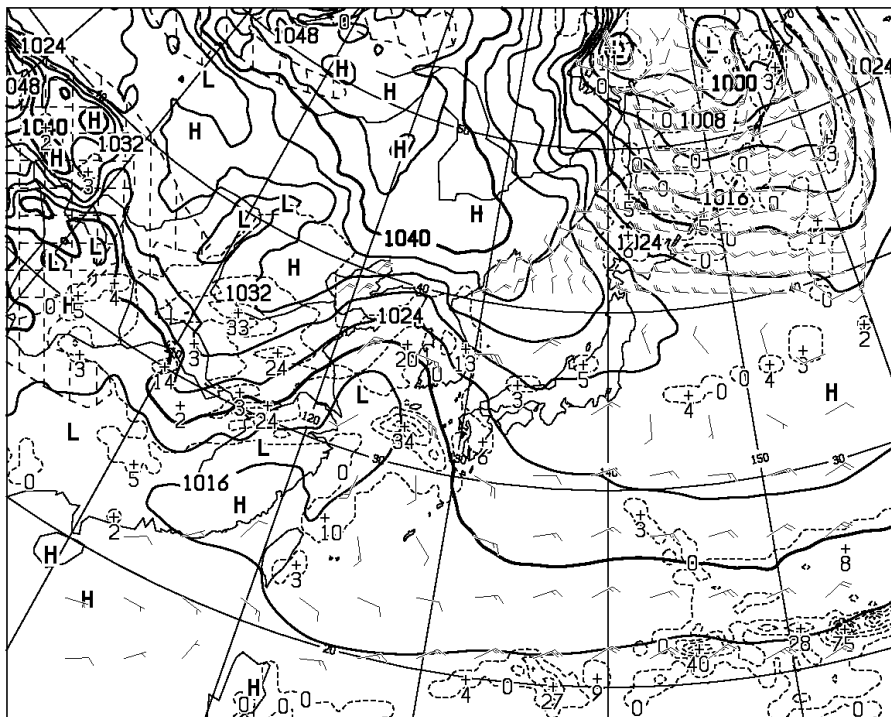
T=36 VALID 110000UTC SURFACE PRESS (hPa), PRECIP (MM) (24-36) WIND ARROW AT SURFACE
