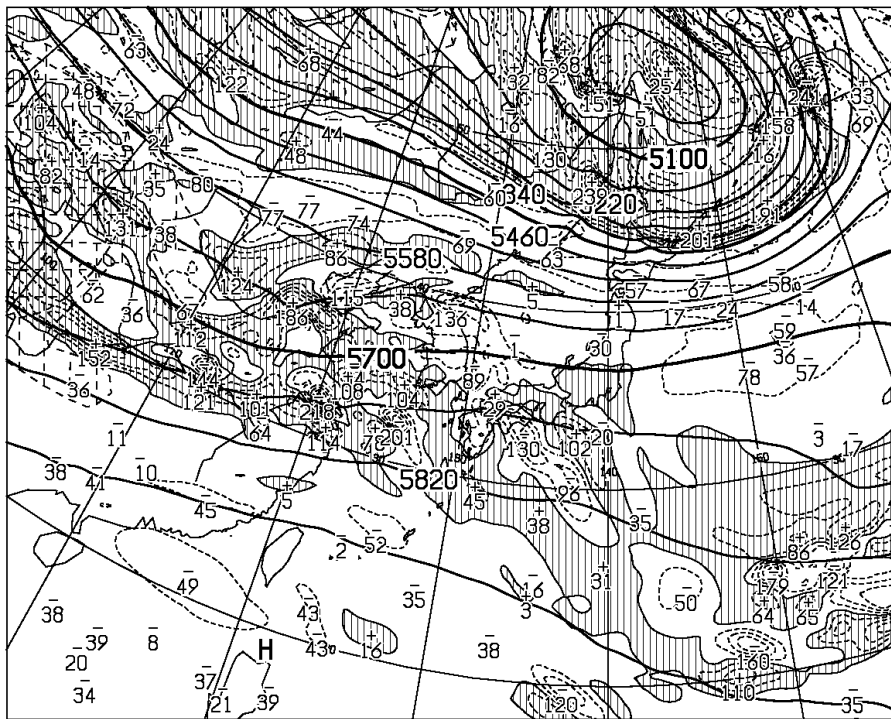
T=36 VALID 110000UTC HEIGHT (M), VORT (10** -6 /SEC) AT 500hPa
