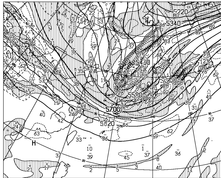
T=48 VALID 191200UTC HEIGHT (M), VORT(10**+6/SEC) AT 500hPa
