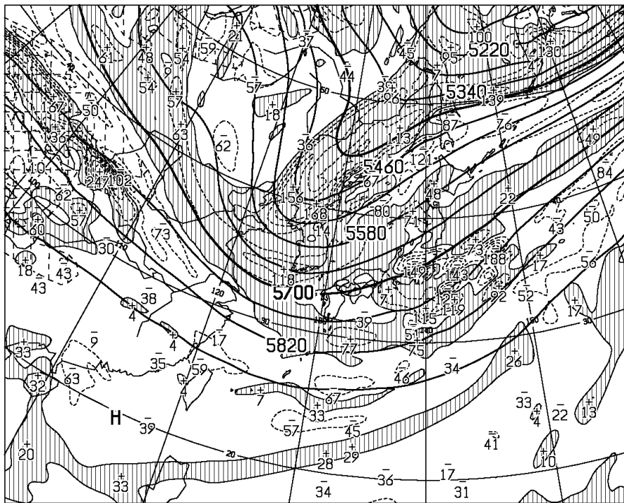
T=36 VALID 190000UTC HEIGHT (M), VORT(10**+6/SEC) AT 500hPa
