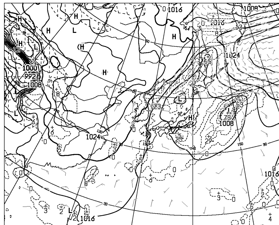
T=48 VALID 191200UTC SURFACE PRESS(hPa), PRECIP (MM) (36-48) WIND ARROW AT SURFACE
