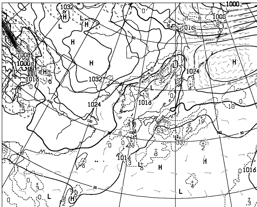
T=36 VALID 190000UTC SURFACE PRESS(hPa), PRECIP (MM) (24-36) WIND ARROW AT SURFACE
