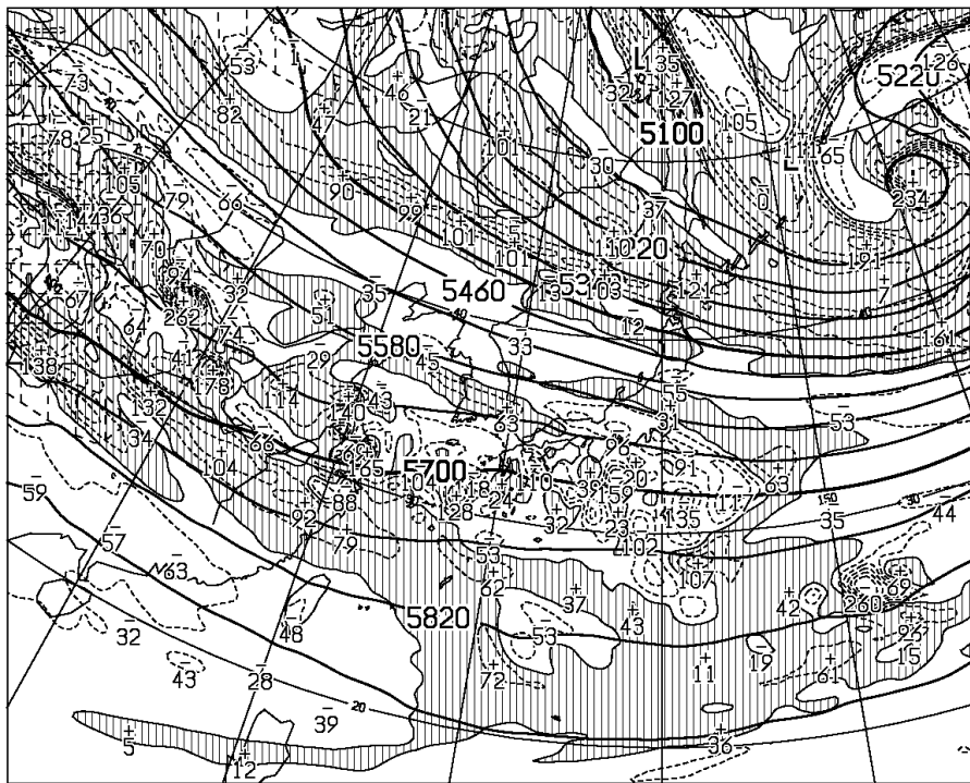
T=36 VALID 050000UTC HEIGHT (M), VORT(10**+6/SEC) AT 500hPa
