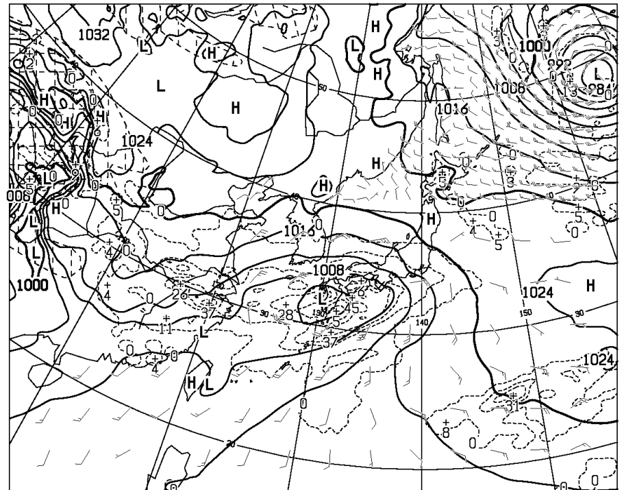
T=48 VALID 051200UTC SURFACE PRESS(hPa), PRECIP (MM) (36-48) WIND ARROW AT SURFACE
