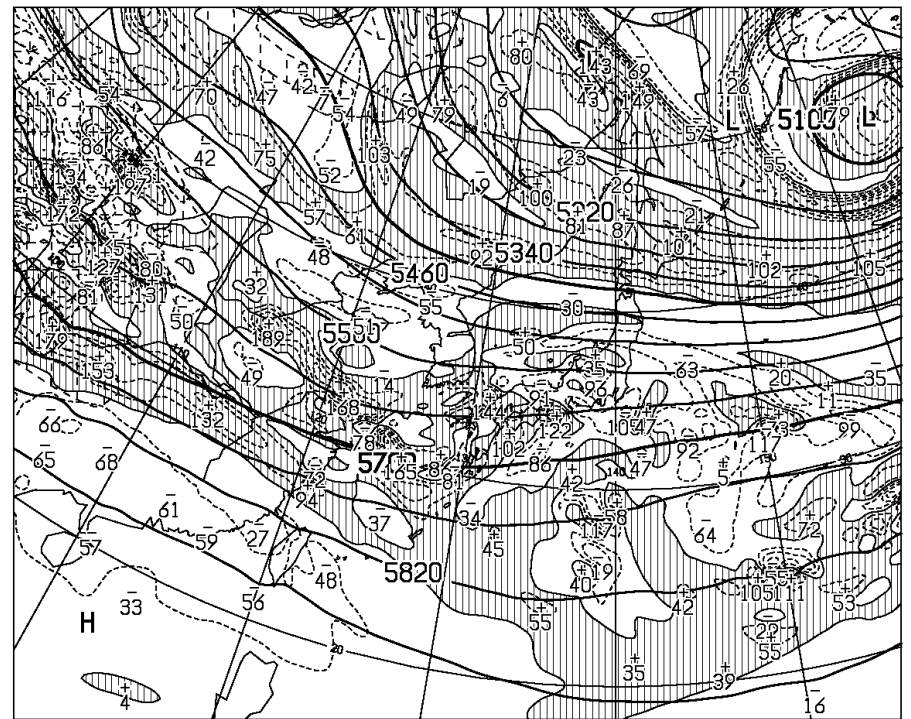
T=48 VALID 051200UTC HEIGHT (M), VORT(10**+6/SEC) AT 500hPa
