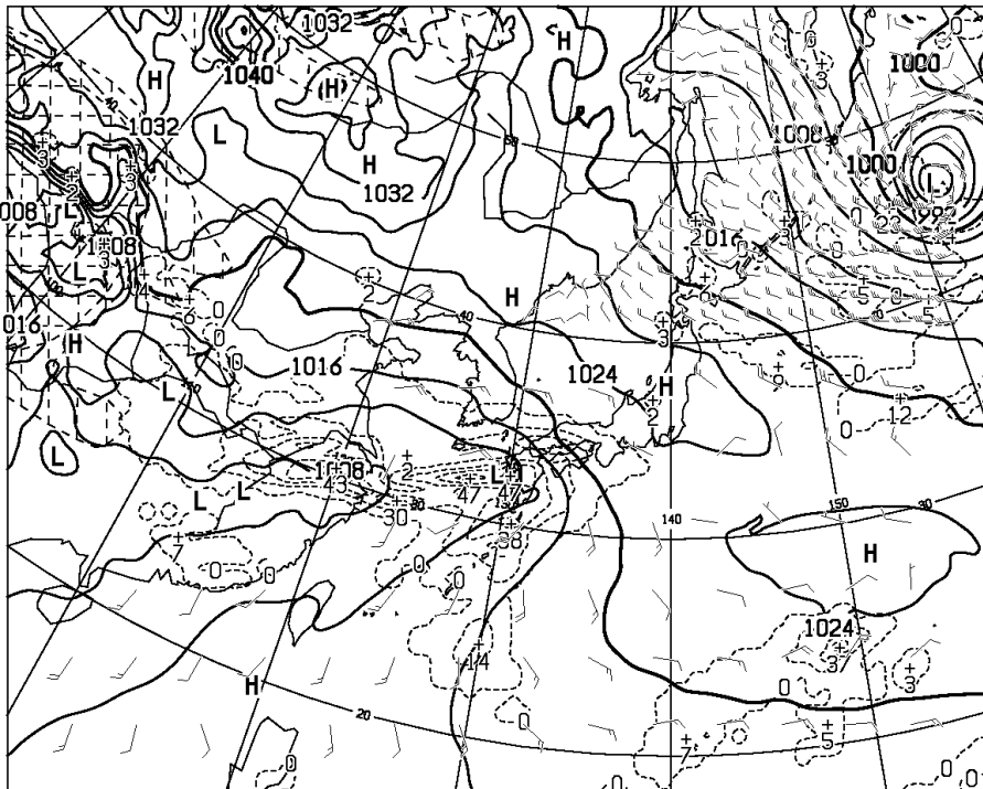
T=36 VALID 050000UTC SURFACE PRESS(hPa), PRECIP (MM) (24-36) WIND ARROW AT SURFACE
