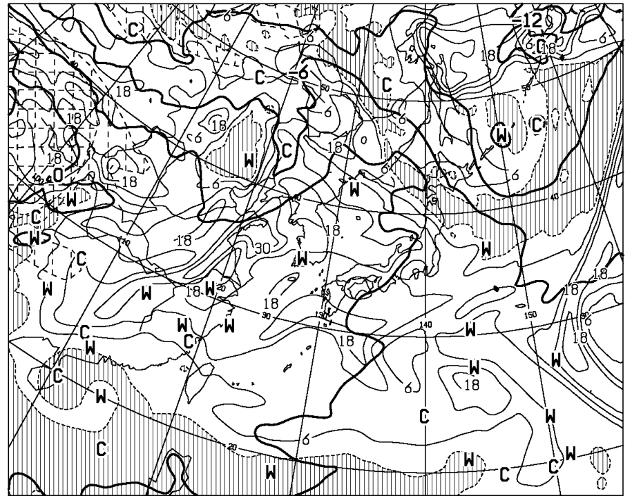
T=24 VALID 171200UTC TEMP (C) AT 500hPa T-TD (C) AT 700hPa
