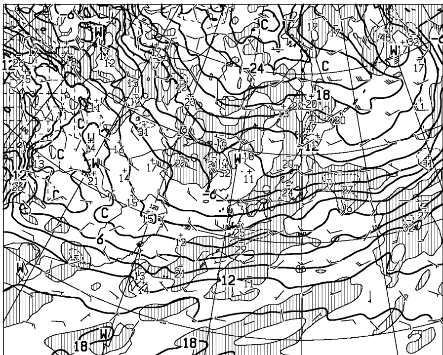
T=12 VALID 221200UTC TEMP (C), WIND ARROW AT 850hPa P-VEL (hPa/h) AT 700hPa
