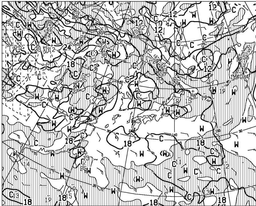
T=12 VALID 170000UTC TEMP (C), WIND ARROW AT 850hPa P-VEL (hPa/h) AT 700hPa
