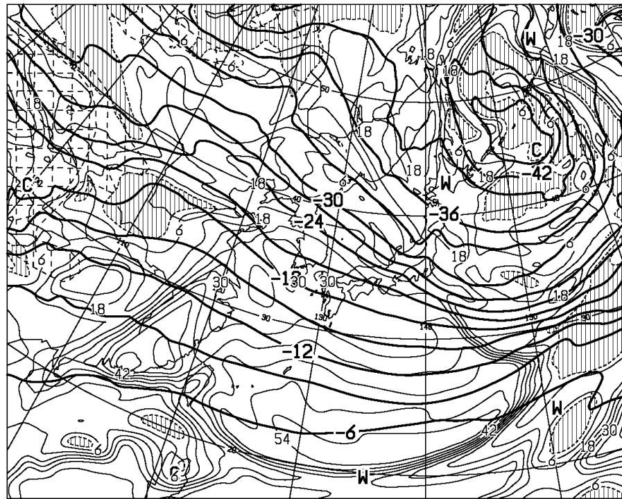
T=24 VALID 181200UTC TEMP (C) AT 500hPa T-TD (C) AT 700hPa
