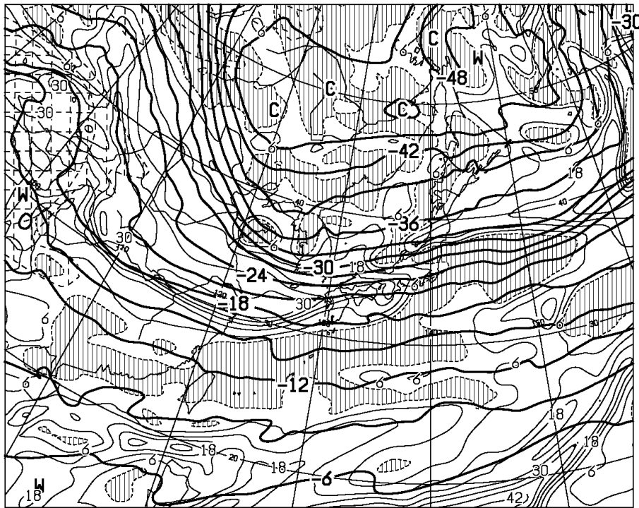
T=12 VALID 221200UTC TEMP (C) AT 500hPa T-TD (C) AT 700hPa
