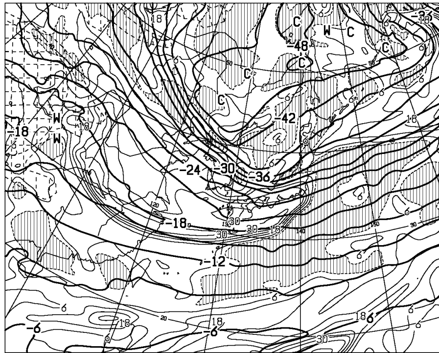
T=24 VALID 230000UTC TEMP (C) AT 500hPa T-TD (C) AT 700hPa
