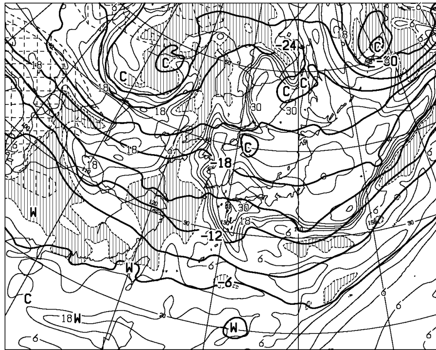
T=24 VALID 220000UTC TEMP (C) AT 500hPa T-TD (C) AT 700hPa
