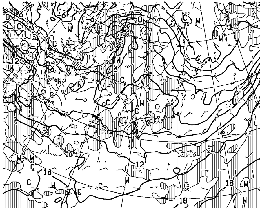
T=24 VALID 220000UTC TEMP (C), WIND ARROW AT 850hPa P-VEL (hPa/h) AT 700hPa
