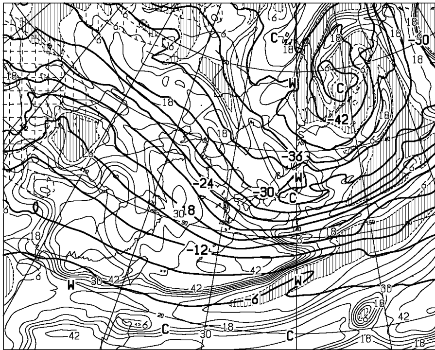
T=12 VALID 180000UTC TEMP (C) AT 500hPa T-TD (C) AT 700hPa
