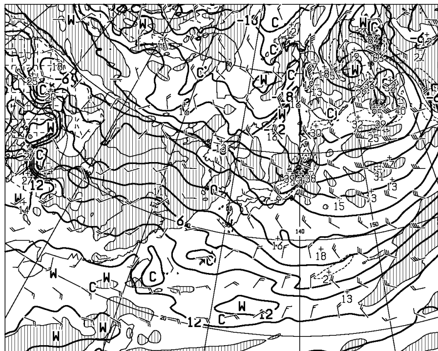
T=24 VALID 181200UTC TEMP (C), WIND ARROW AT 850hPa P-VEL (hPa/h) AT 700hPa
