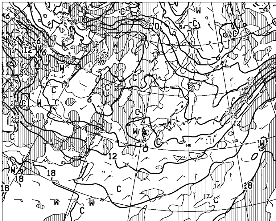
T=12 VALID 211200UTC TEMP (C), WIND ARROW AT 850hPa P-VEL (hPa/h) AT 700hPa
