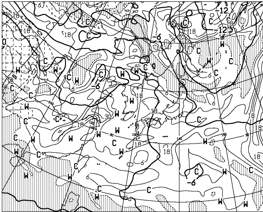
T=12 VALID 170000UTC TEMP (C) AT 500hPa T-TD (C) AT 700hPa
