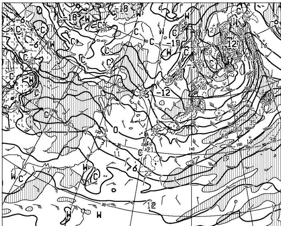
T=12 VALID 180000UTC TEMP (C), WIND ARROW AT 850hPa P-VEL (hPa/h) AT 700hPa
