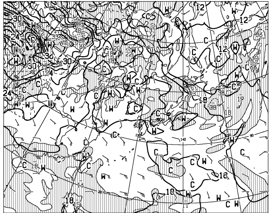
T=24 VALID 171200UTC TEMP (C), WIND ARROW AT 850hPa P-VEL (hPa/h) AT 700hPa
