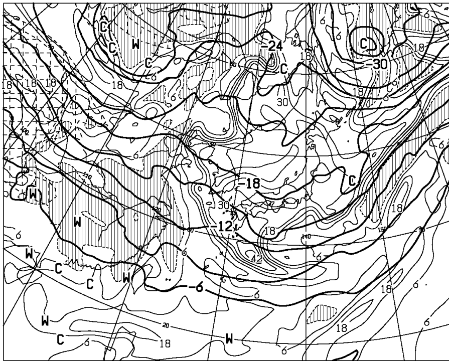
T=12 VALID 211200UTC TEMP (C) AT 500hPa T-TD (C) AT 700hPa
