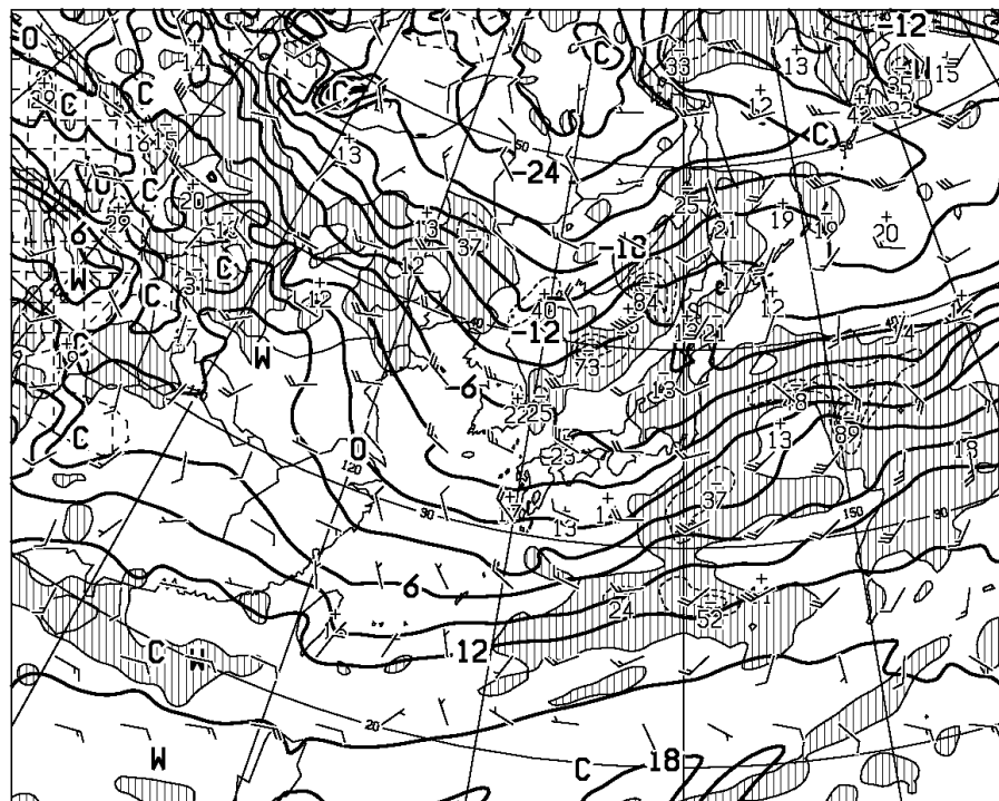
T=24 VALID 230000UTC TEMP (C), WIND ARROW AT 850hPa P-VEL (hPa/h) AT 700hPa
